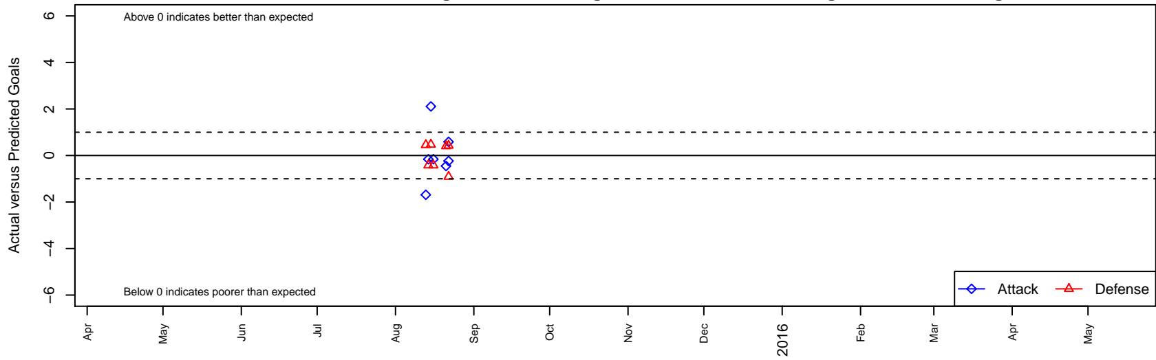
Seattle United S Blue G97 Dots are actual minus expected GF (blue circles) and GA (red triangles). Blue line is smoothed change in attack strength. Red is smoothed change in defense strength.
